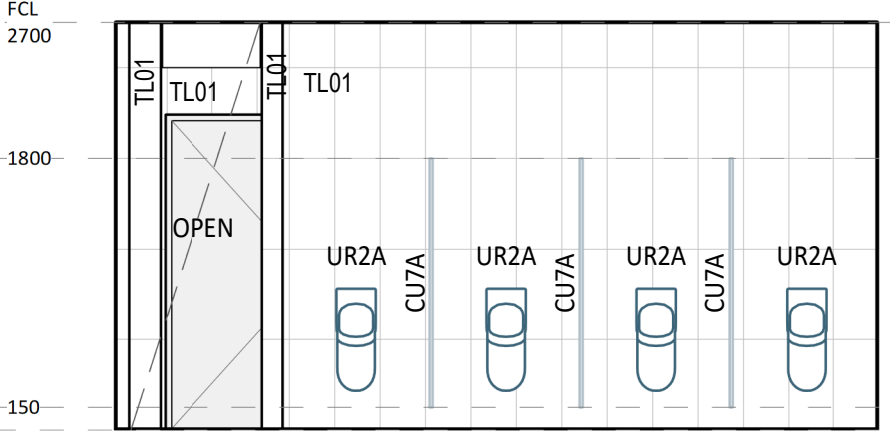
4 ELEVATION DETAIL 60-130 1 : 50
