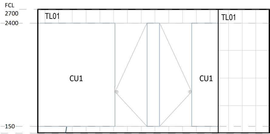
2 ELEVATION DETAIL 60-130 1 : 50
