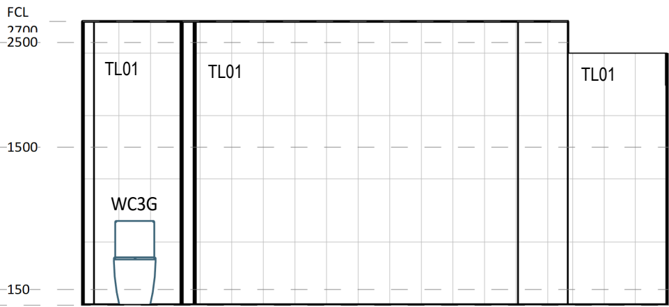
3 ELEVATION DETAIL 60-037 1 : 50
