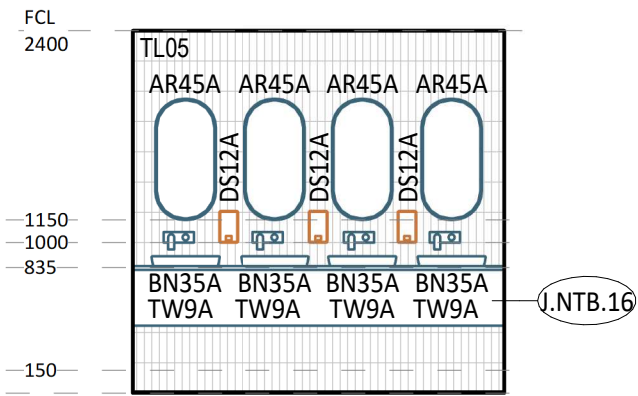
5 ELEVATION DETAIL 60-036 1 : 50
