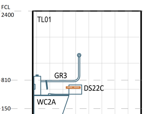
7 ELEVATION DETAIL 60-130 1 : 50
