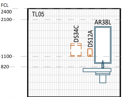
9 ELEVATION DETAIL 60-130 1 : 50
